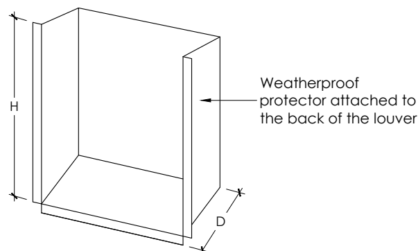
Weatherproof protector
