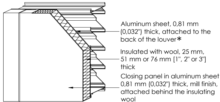
Insulated blankoff panel
