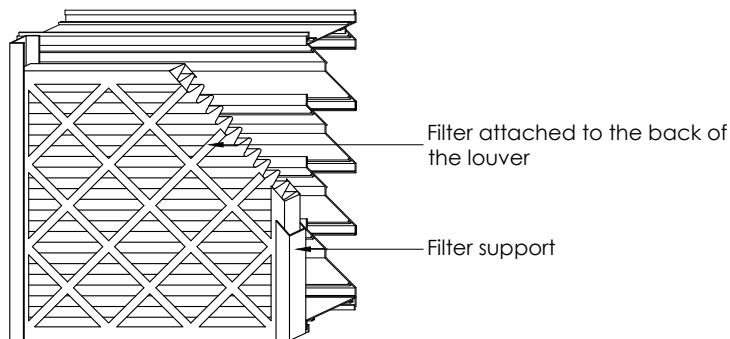
Replaceable filters
