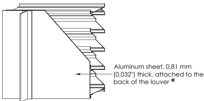
Non-insulated blankoff panel
