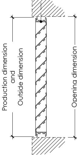
"U" frame (CU)
