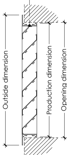
"L" frame (CL)
